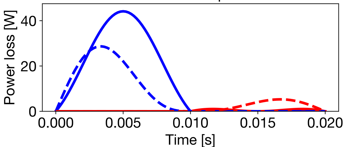
Total IGBT and diode power losses
