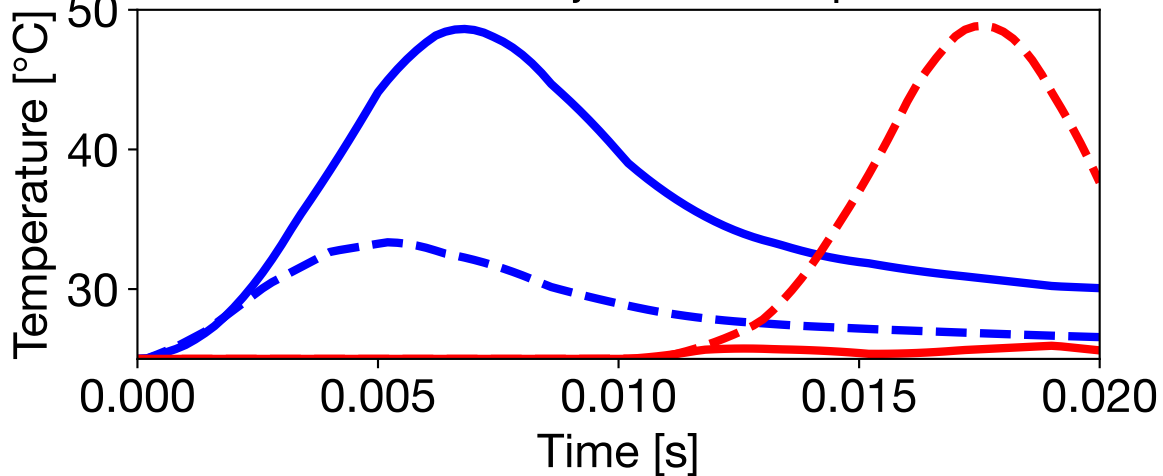
IGBT and diode junction temperature
