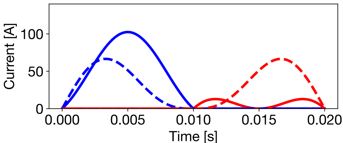
Instantaneous IGBT and diode currents
